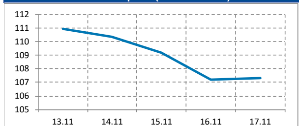
Steinkohlepreis (ICE Coal 2024)
