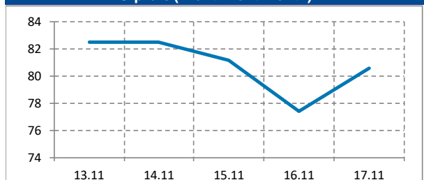
Ölpreis (Brent Front Month)
